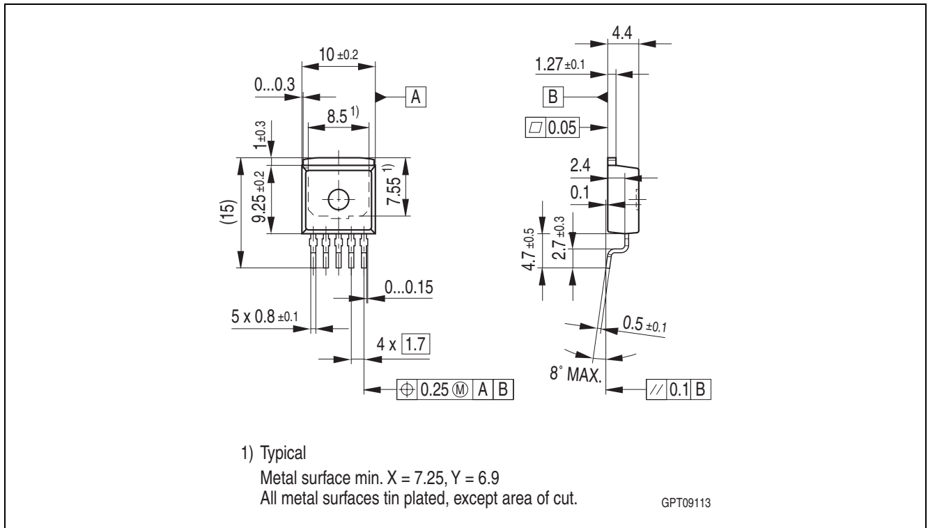
Figure 7 PG-TO263-5
