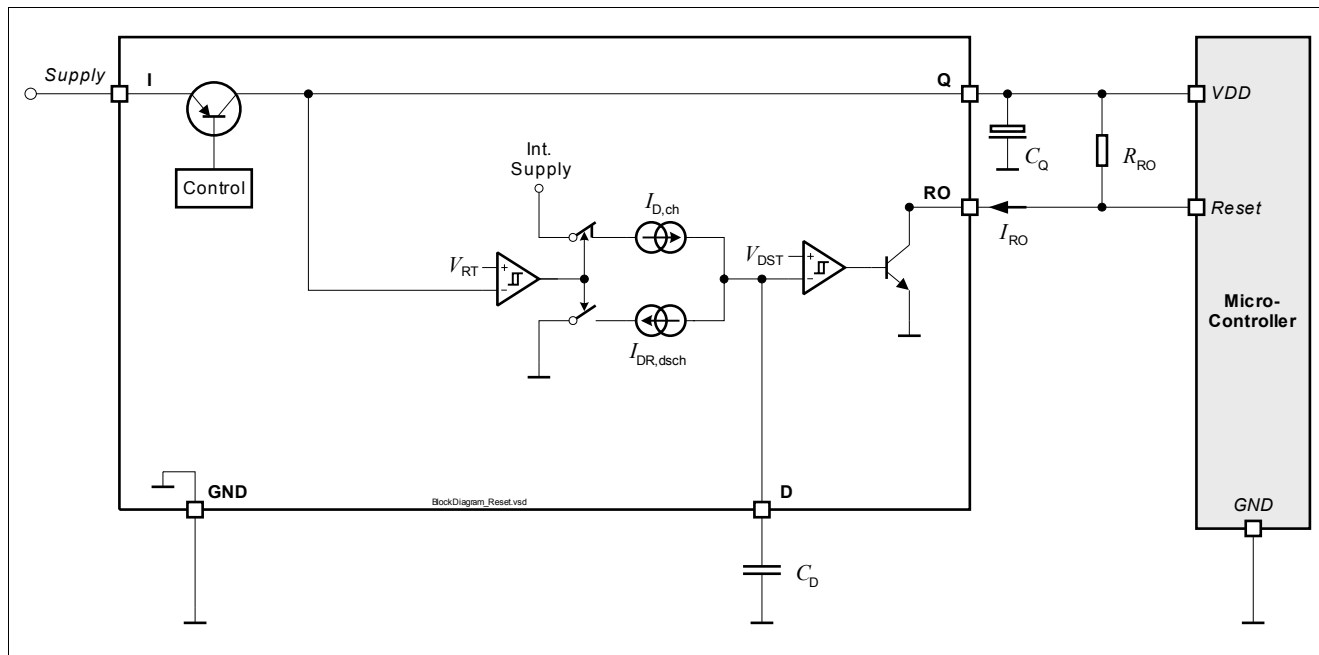
Figure 4 Block Diagram Reset Function
